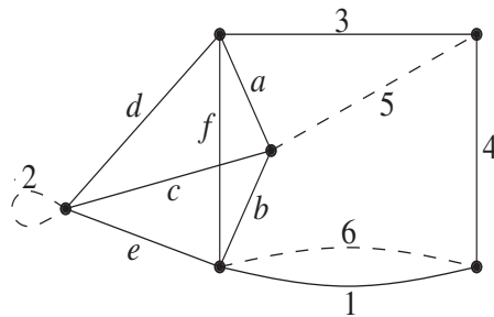
FIG. 4.1. Signed-graphic representation of M_{12} . Negative edges are dashed; positive edges are solid.
